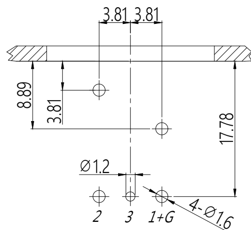
PCB-Layout(component side)
