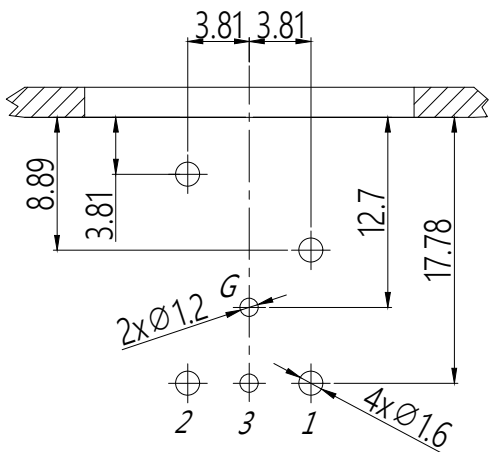
PCB-Layout(component side)
