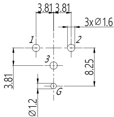
PCB-Layout(component side)
