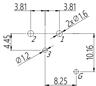
PCB-Layout(component side)
