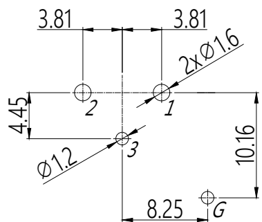
PCB-Layout(component side)
