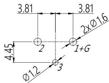
PCB-Layout(component side)
