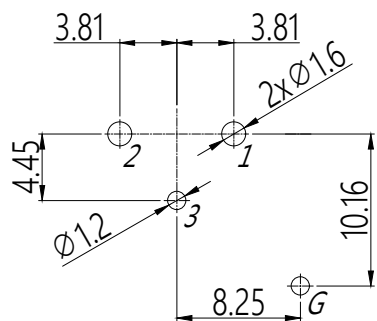
PCB-Layout(component side)
