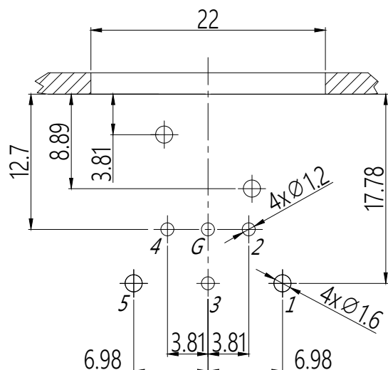
PCB-Layout(component side)
