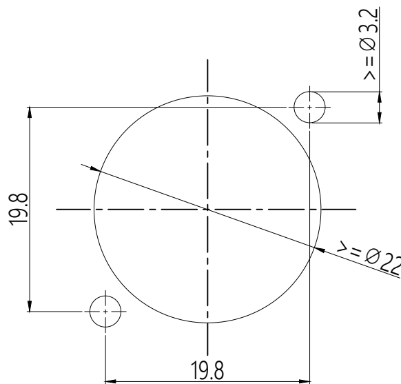
Panel cut out(Rear side)
