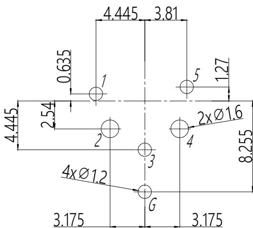
PCB-LAYOUT(component side)
