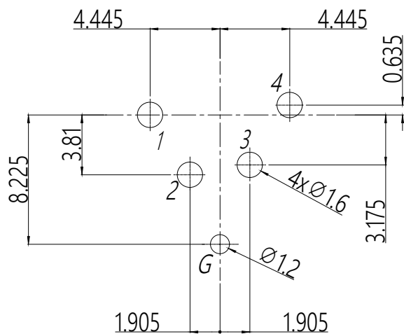
PCB-Layout(component side)
