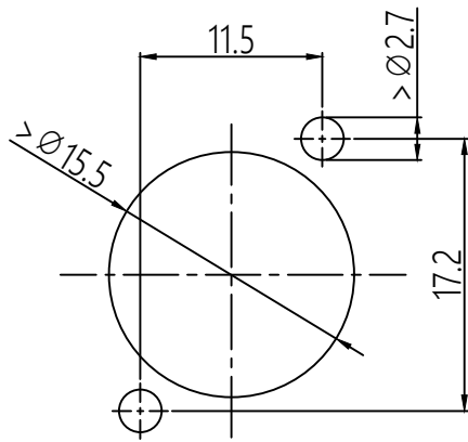
Panel cut out (Rear side)
